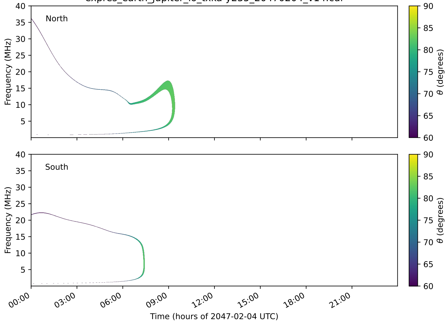
expres_earth_jupiter_io_txka-y235_20470204_v14.cdf
