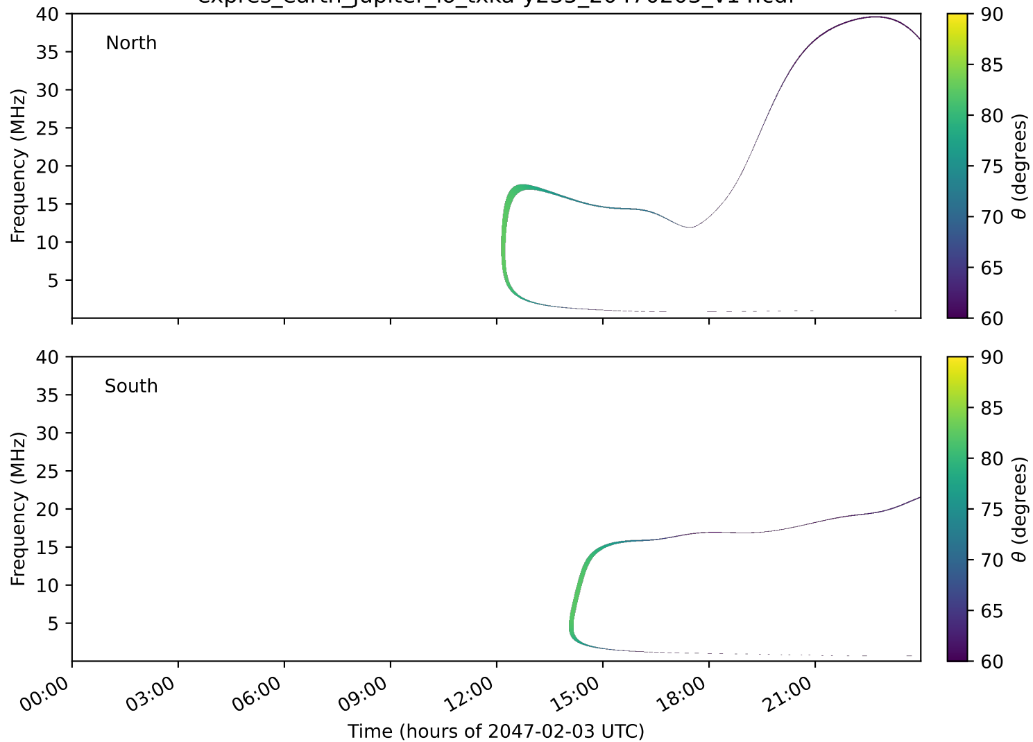
expres_earth_jupiter_io_txka-y235_20470203_v14.cdf
