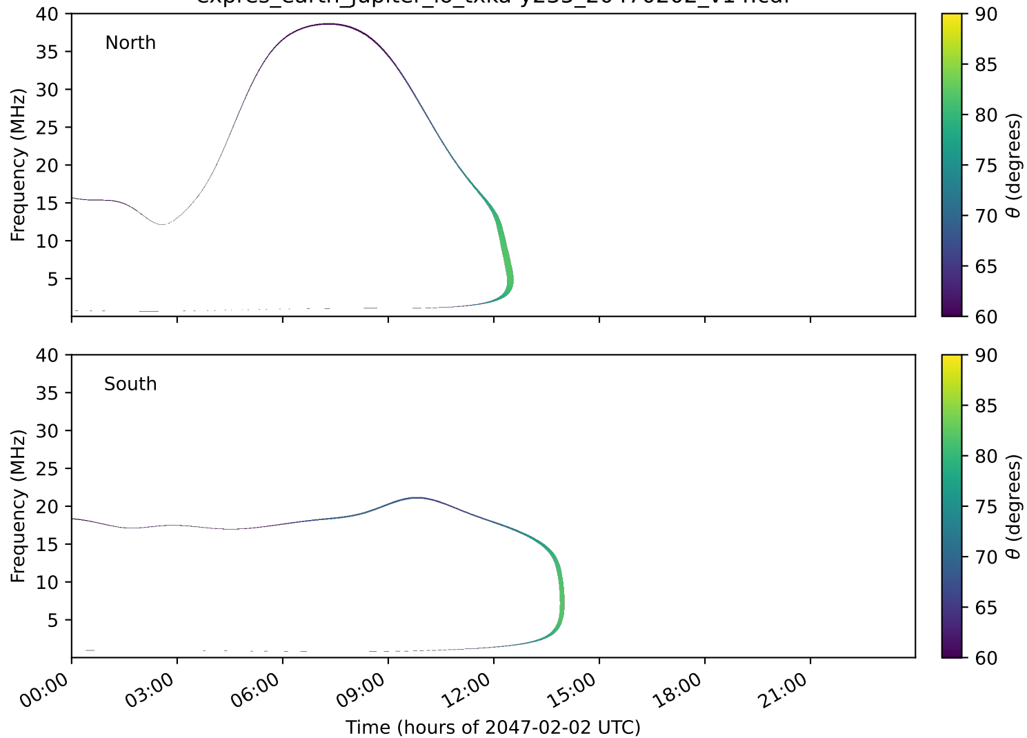
expres_earth_jupiter_io_txka-y235_20470202_v14.cdf
