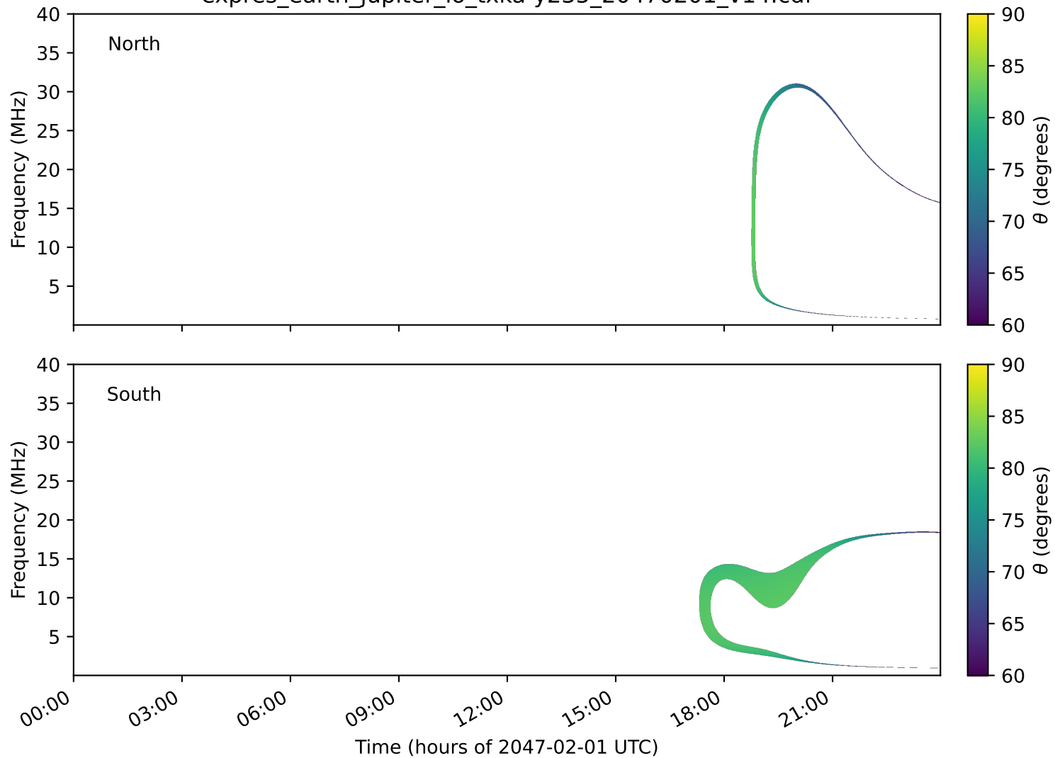
expres_earth_jupiter_io_txka-y235_20470201_v14.cdf
