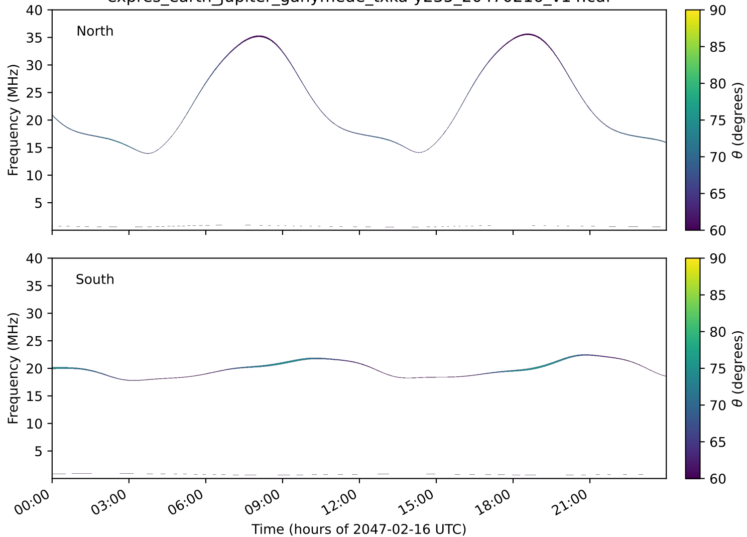
expres_earth_jupiter_ganymede_txka-y235_20470216_v14.cdf
