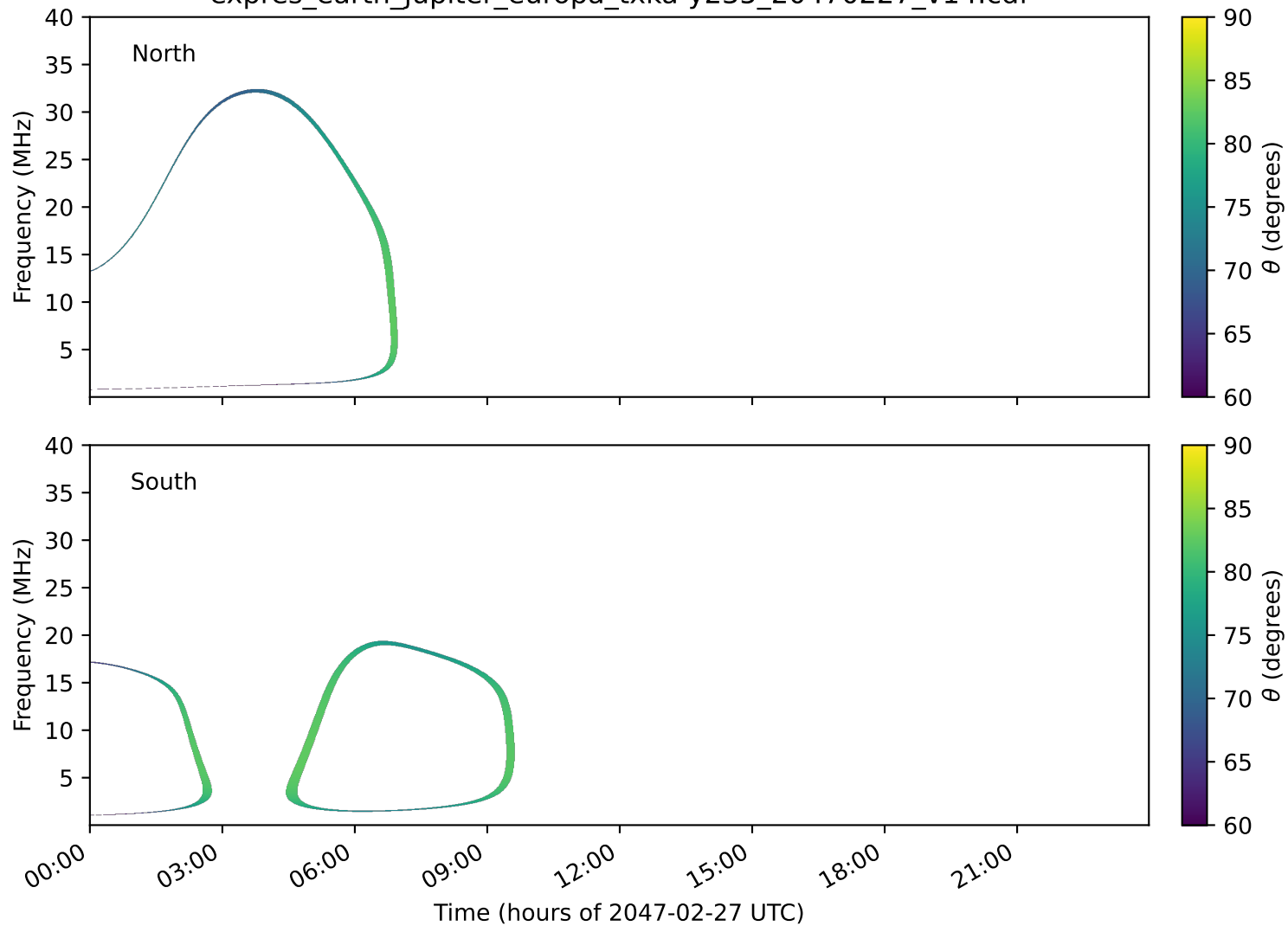
expres_earth_jupiter_europa_txka-y235_20470227_v14.cdf
