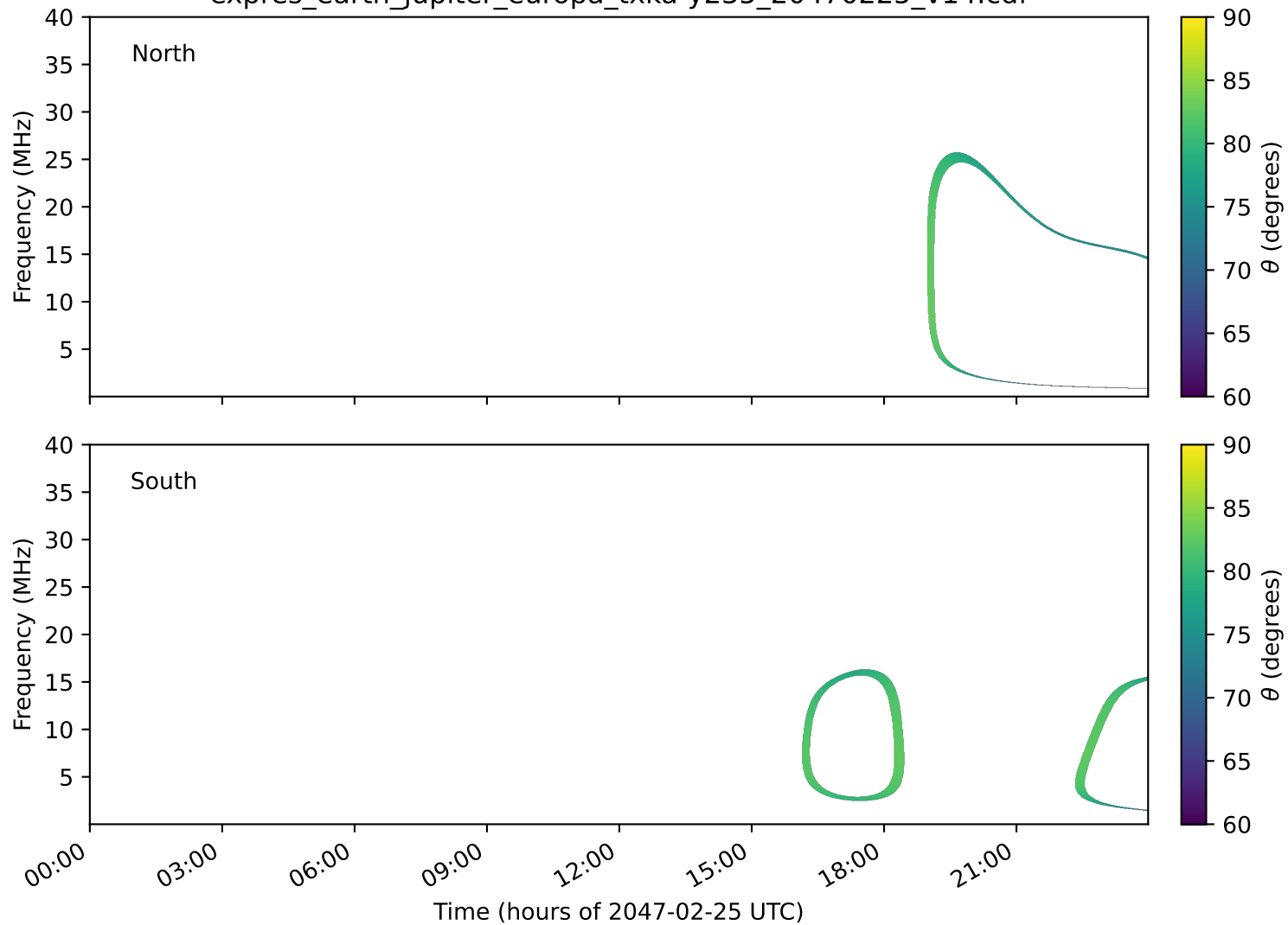
expres_earth_jupiter_europa_txka-y235_20470225_v14.cdf
