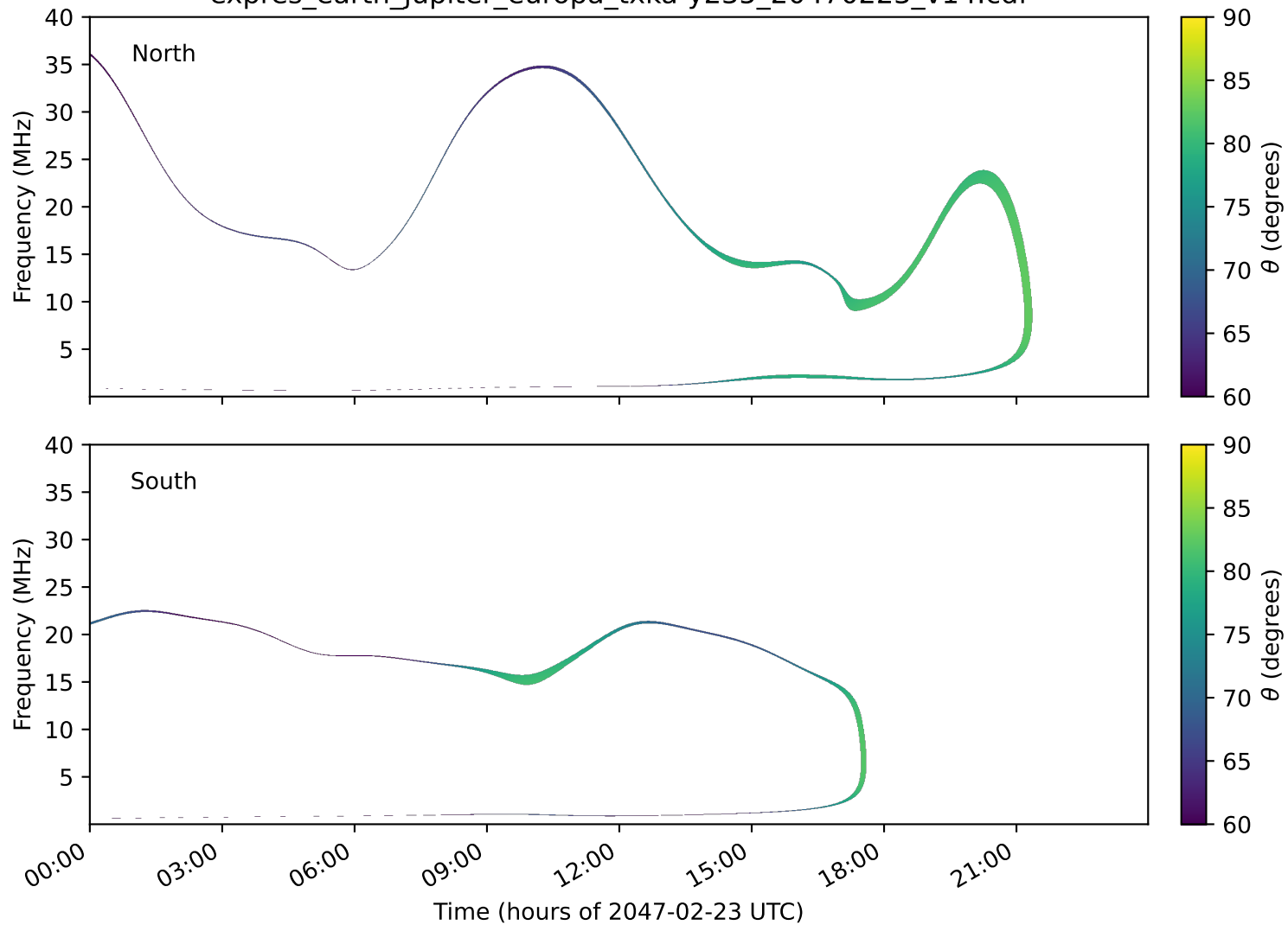
expres_earth_jupiter_europa_txka-y235_20470223_v14.cdf
