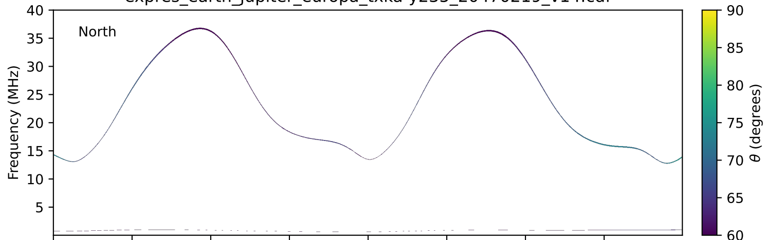
expres_earth_jupiter_europa_txka-y235_20470219_v14.cdf
