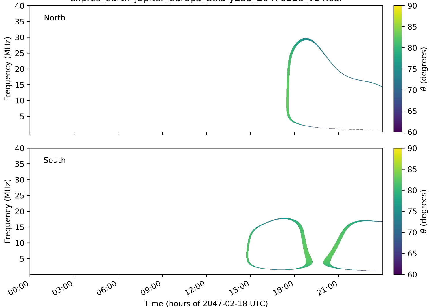
expres_earth_jupiter_europa_txka-y235_20470218_v14.cdf
