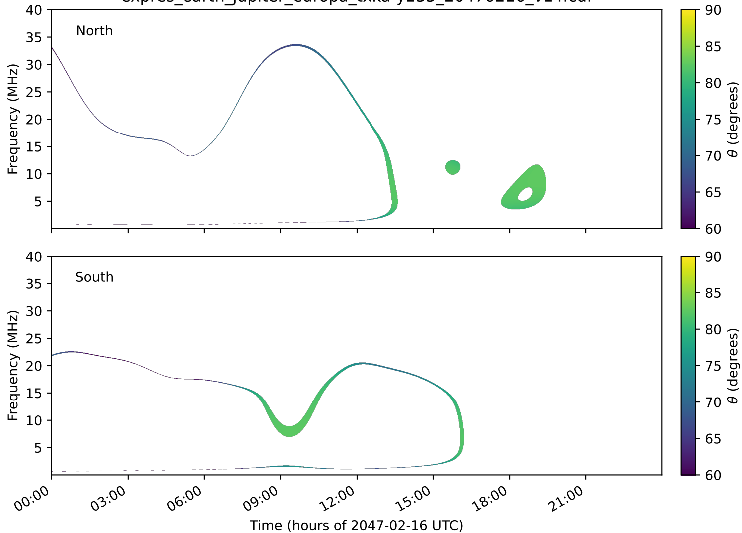
expres_earth_jupiter_europa_txka-y235_20470216_v14.cdf
