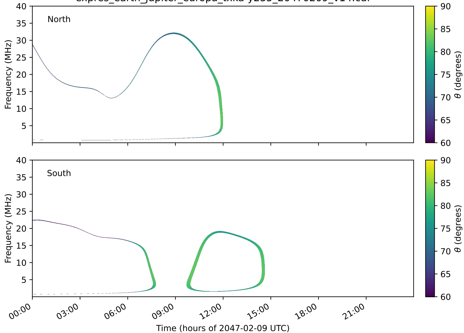
expres_earth_jupiter_europa_txka-y235_20470209_v14.cdf
