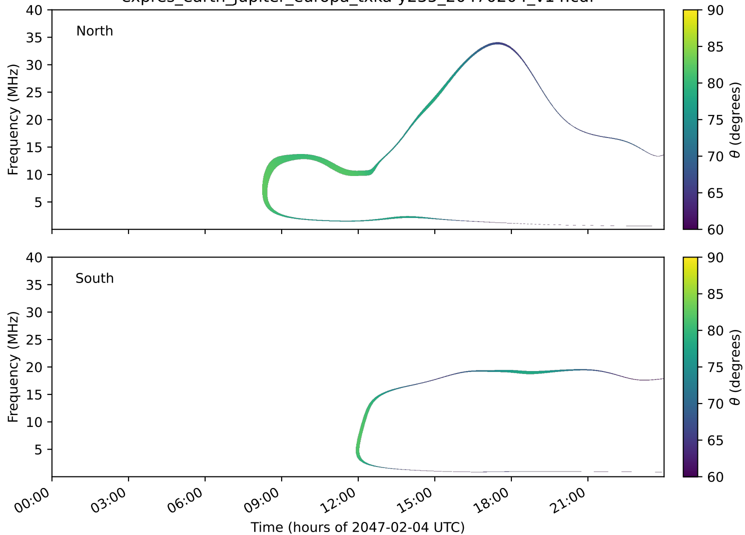
expres_earth_jupiter_europa_txka-y235_20470204_v14.cdf
