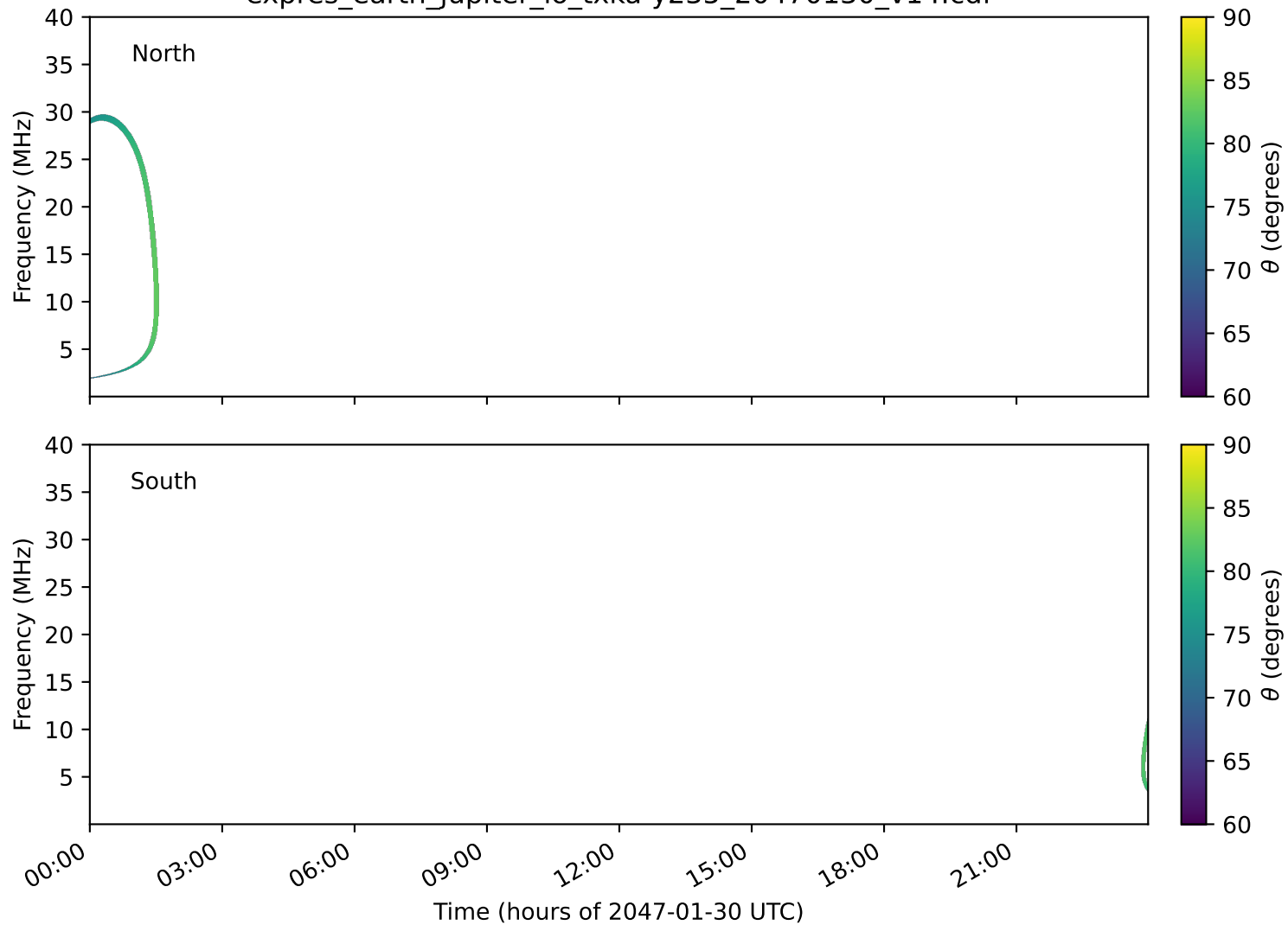
expres_earth_jupiter_io_txka-y235_20470130_v14.cdf
