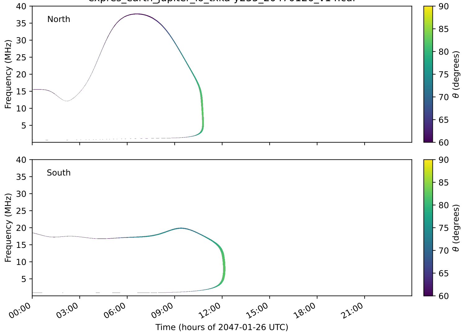
expres_earth_jupiter_io_txka-y235_20470126_v14.cdf
