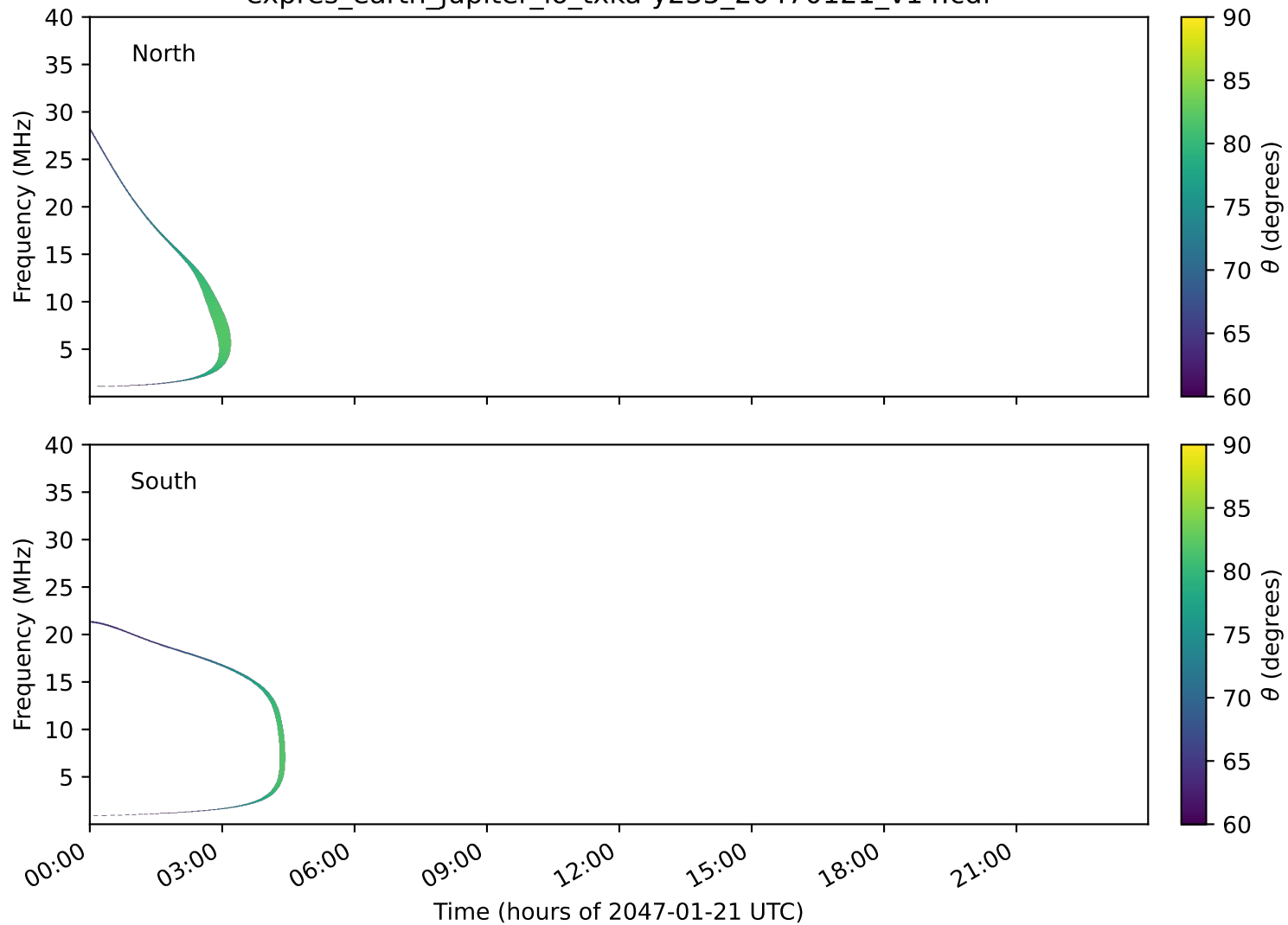
expres_earth_jupiter_io_txka-y235_20470121_v14.cdf
