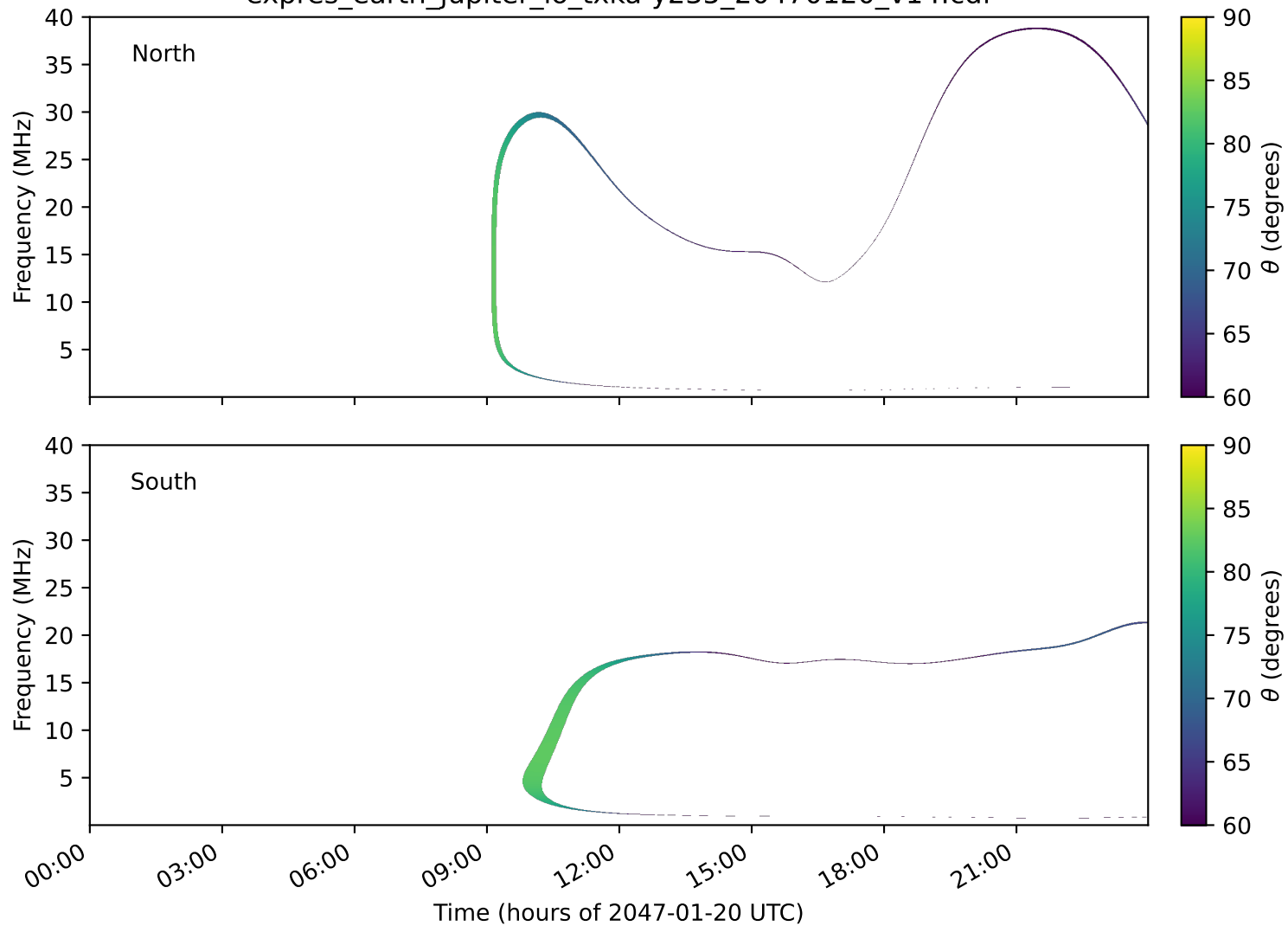
expres_earth_jupiter_io_txka-y235_20470120_v14.cdf
