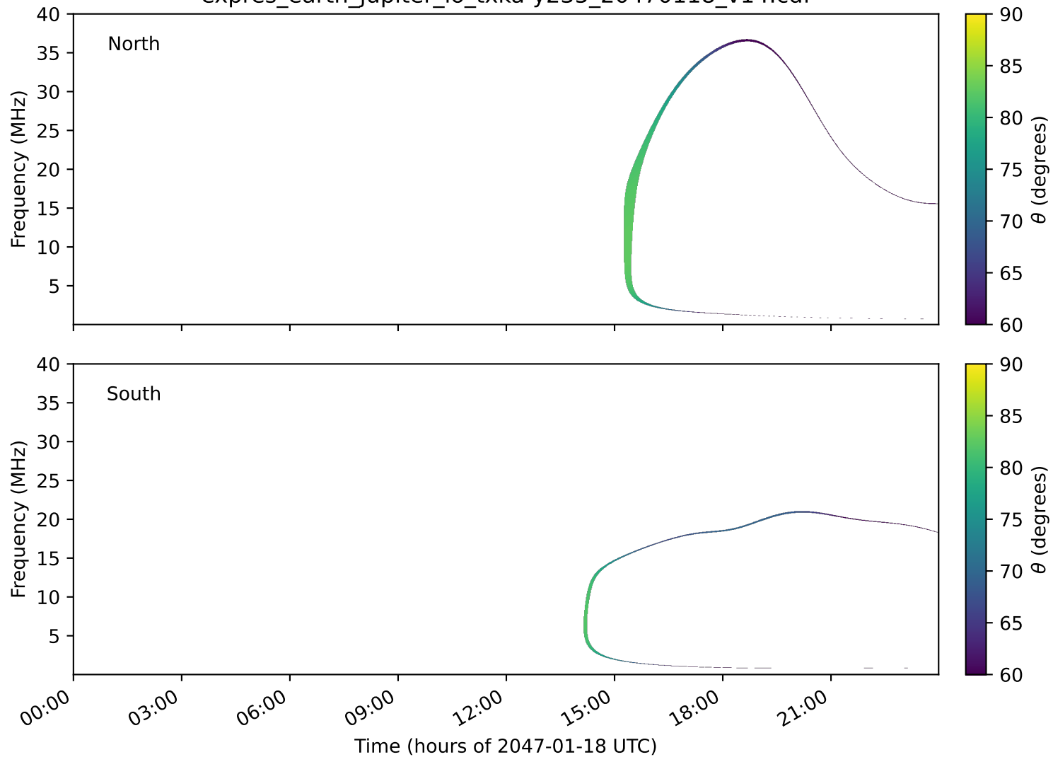
expres_earth_jupiter_io_txka-y235_20470118_v14.cdf
