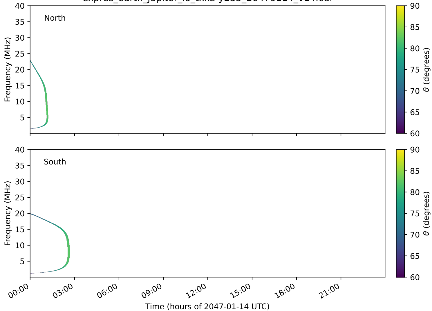
expres_earth_jupiter_io_txka-y235_20470114_v14.cdf
