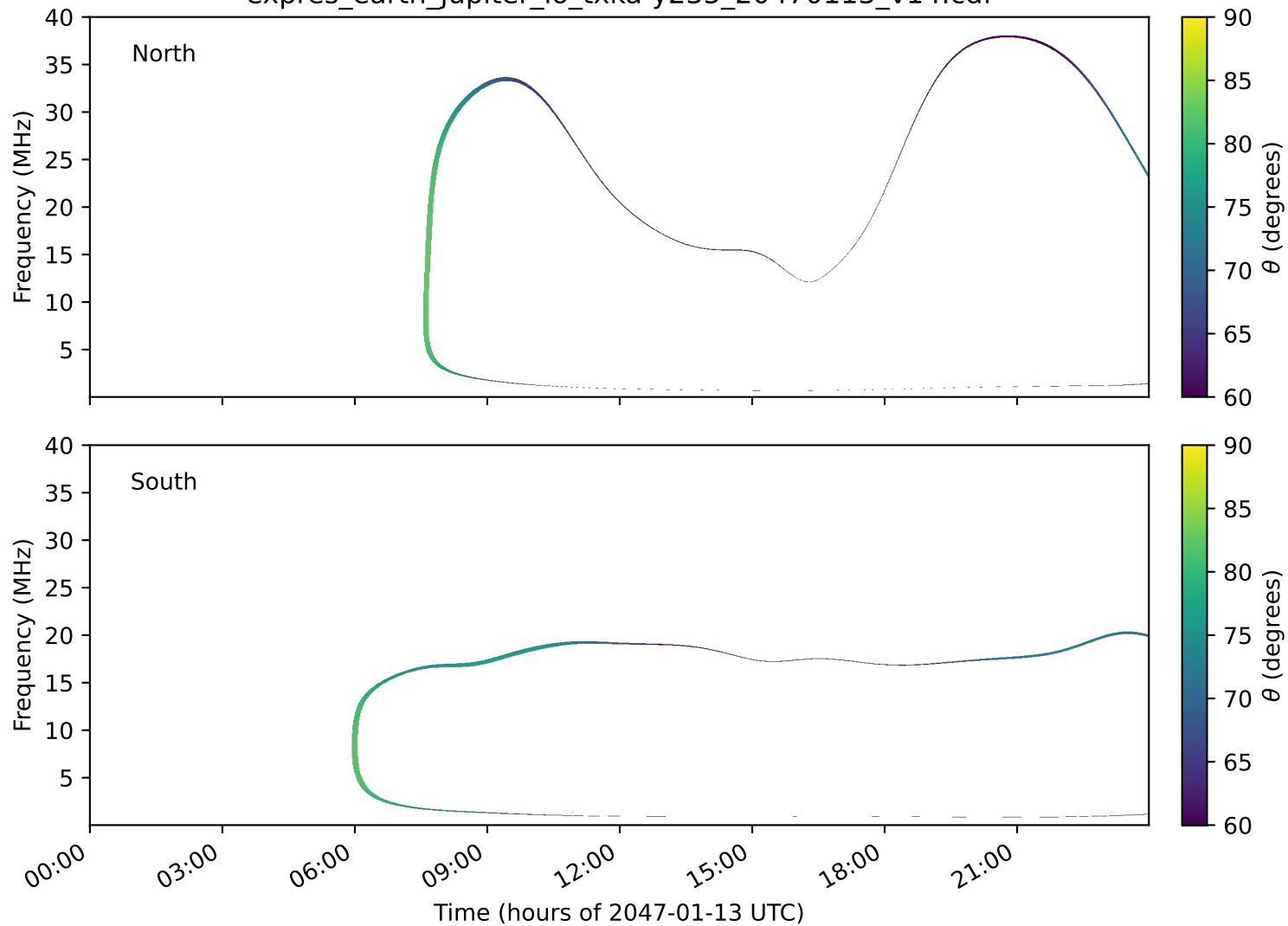
expres_earth_jupiter_io_txka-y235_20470113_v14.cdf
