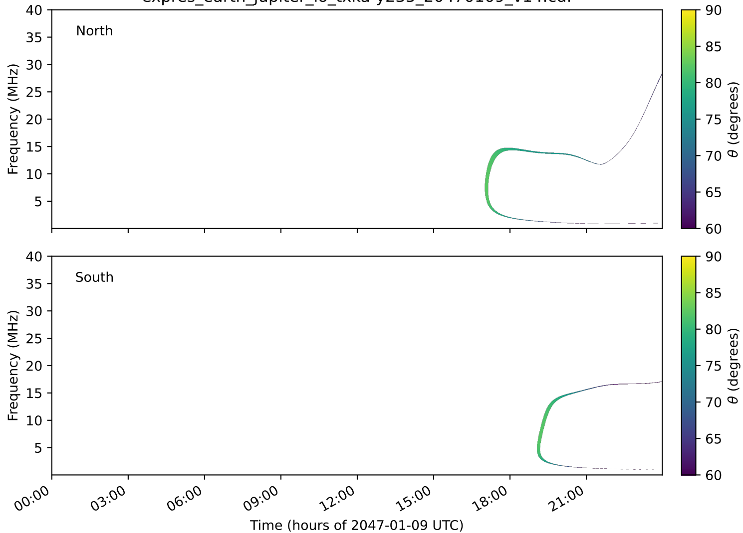
expres_earth_jupiter_io_txka-y235_20470109_v14.cdf
