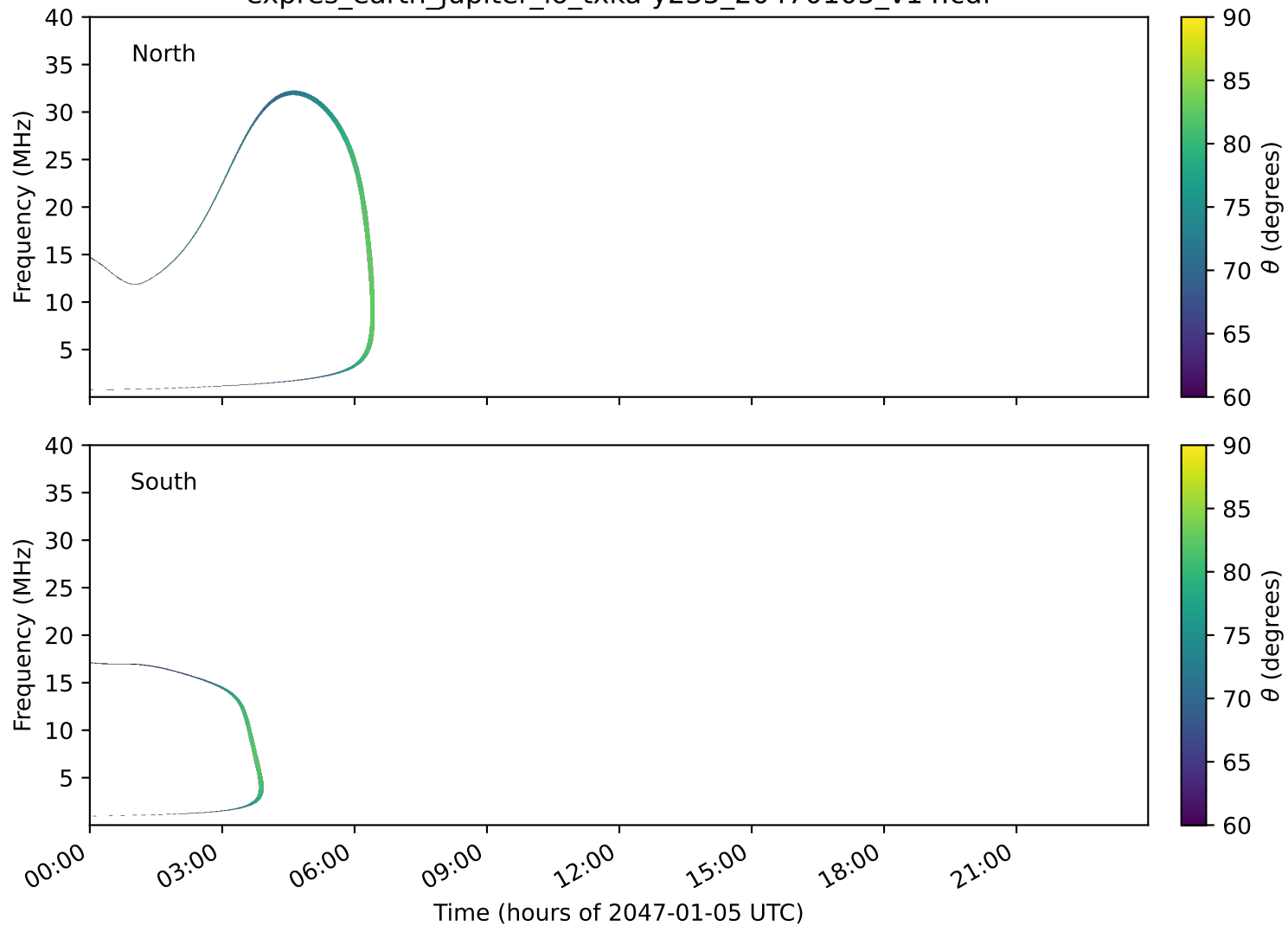
expres_earth_jupiter_io_txka-y235_20470105_v14.cdf
