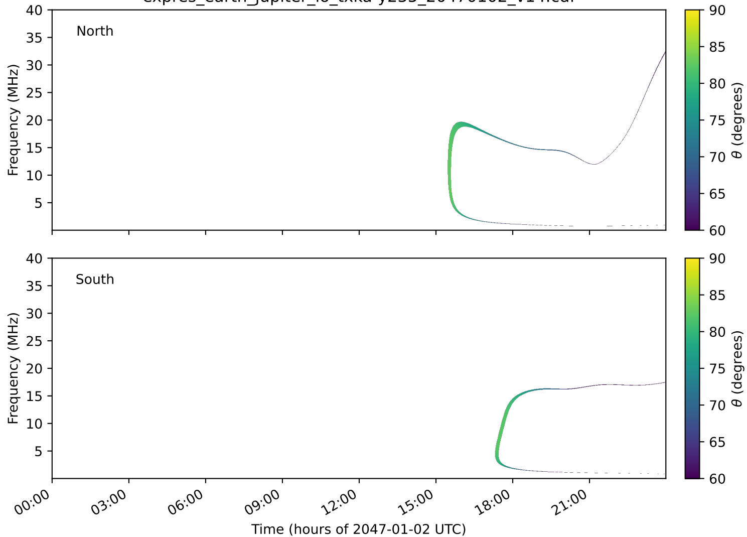
expres_earth_jupiter_io_txka-y235_20470102_v14.cdf
