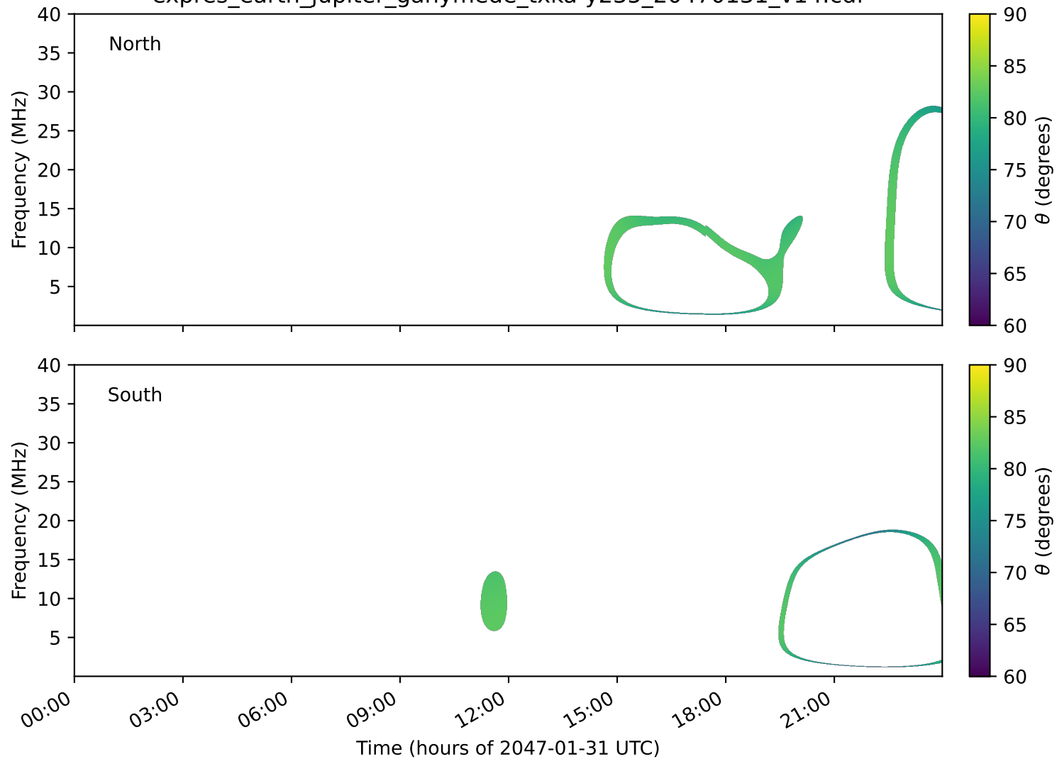
expres_earth_jupiter_ganymede_txka-y235_20470131_v14.cdf
