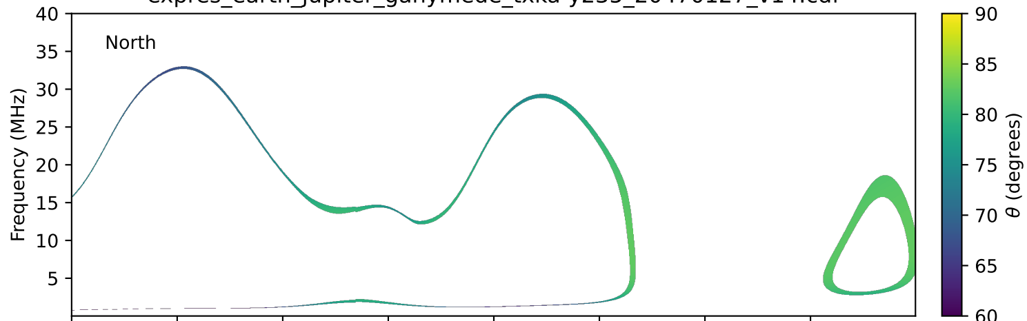
expres_earth_jupiter_ganymede_txka-y235_20470127_v14.cdf
