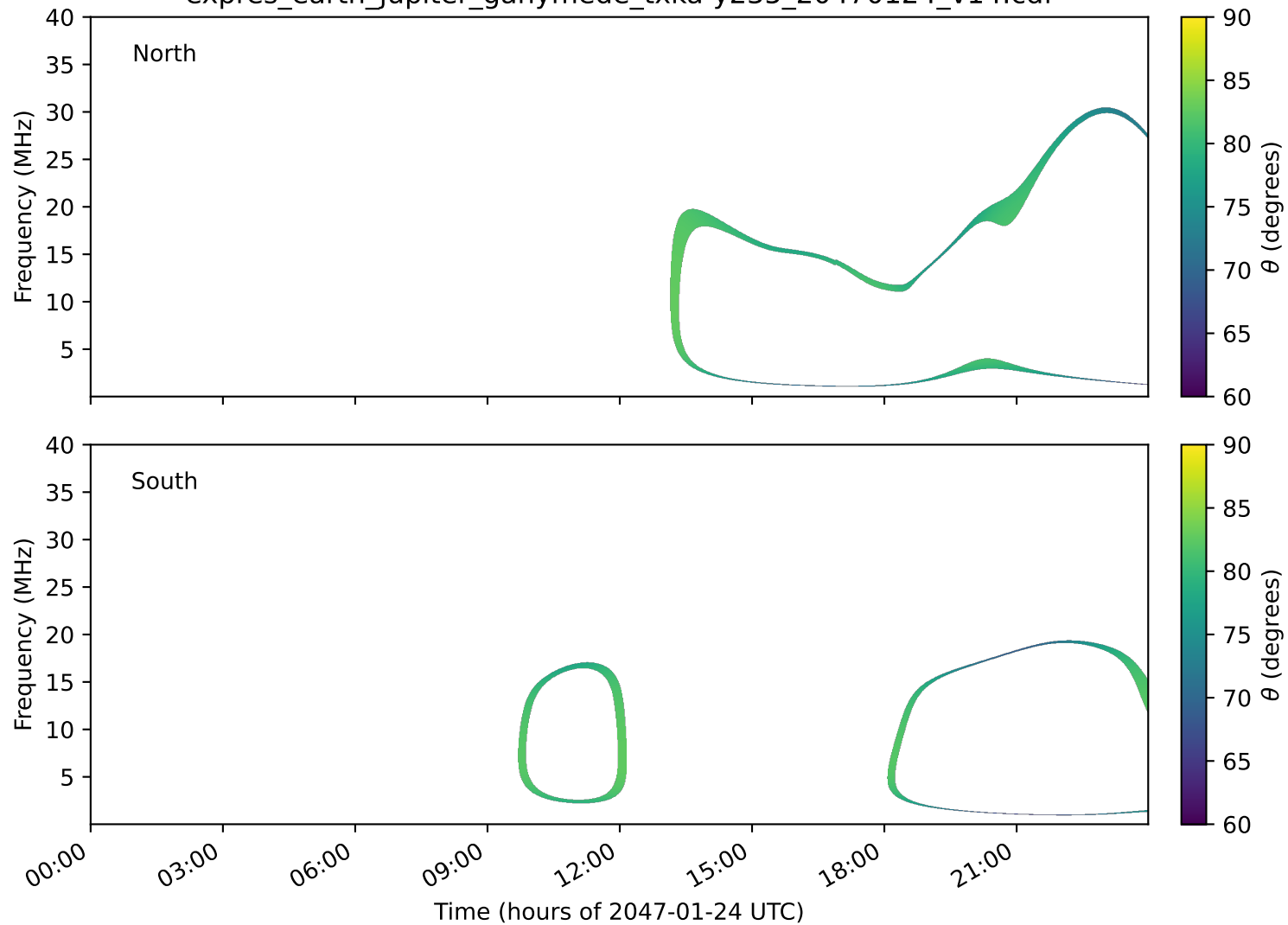
expres_earth_jupiter_ganymede_txka-y235_20470124_v14.cdf
