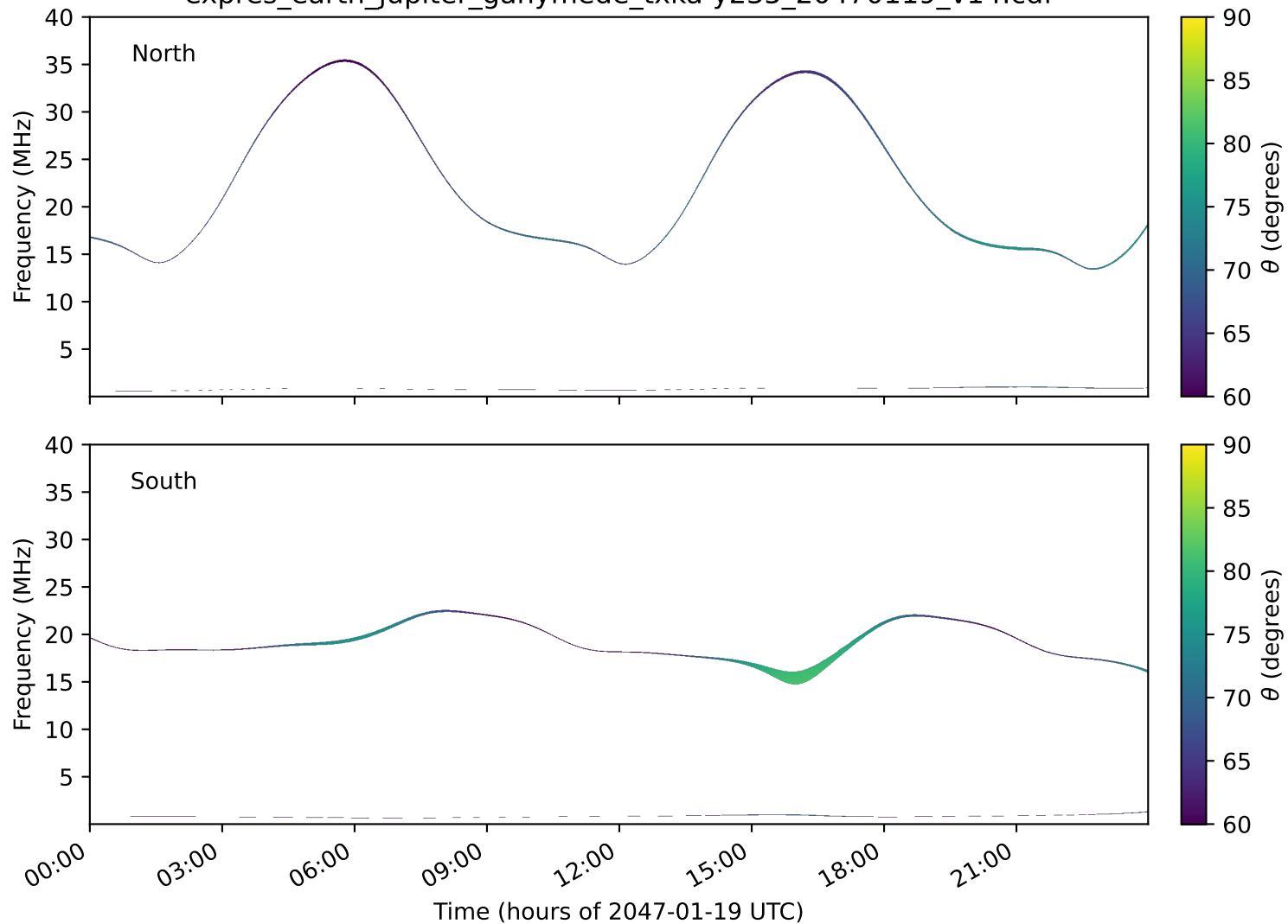
expres_earth_jupiter_ganymede_txka-y235_20470119_v14.cdf
