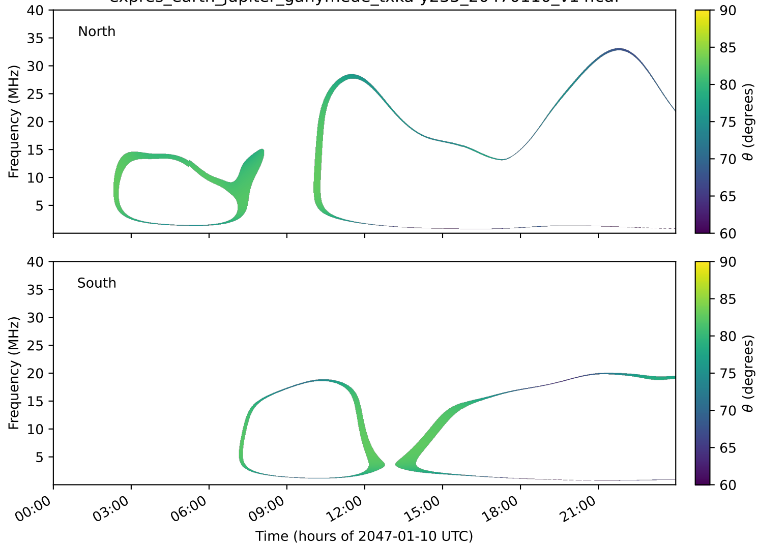
expres_earth_jupiter_ganymede_txka-y235_20470110_v14.cdf
