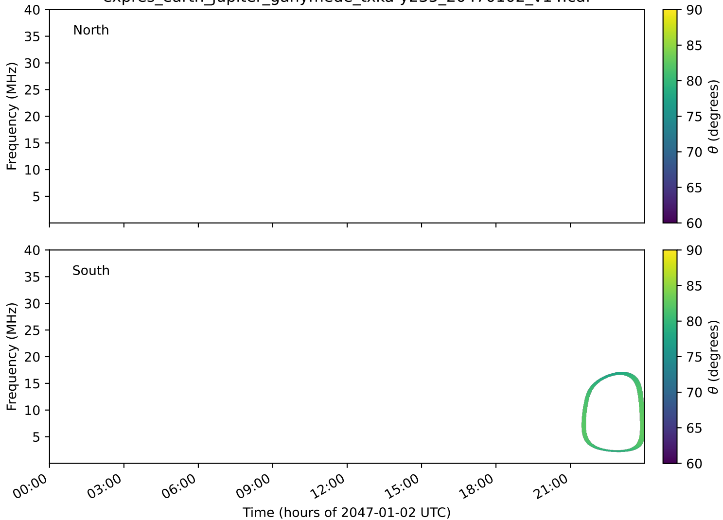
expres_earth_jupiter_ganymede_txka-y235_20470102_v14.cdf
