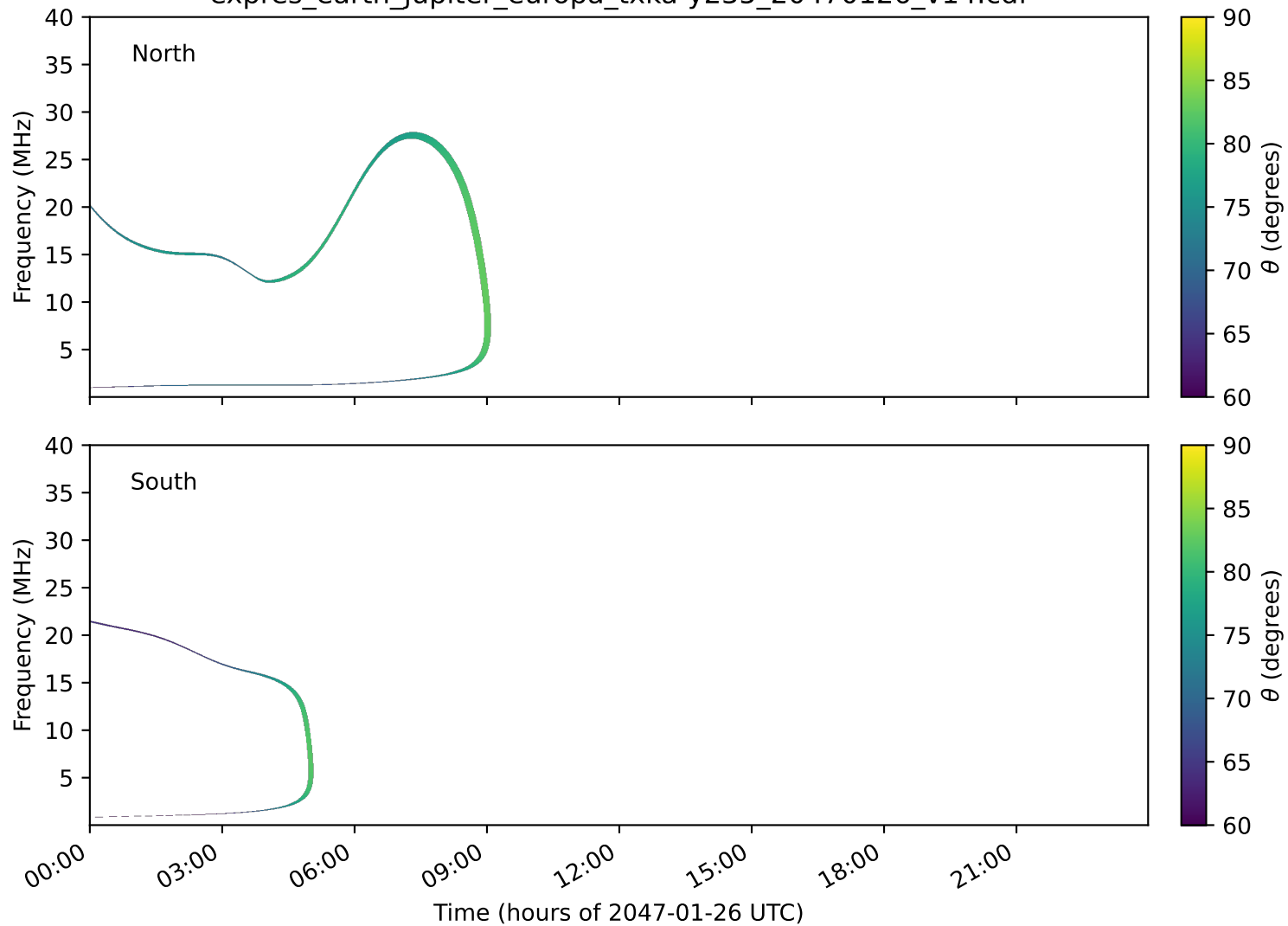
expres_earth_jupiter_europa_txka-y235_20470126_v14.cdf
