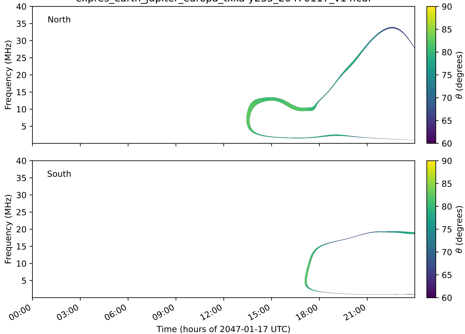
expres_earth_jupiter_europa_txka-y235_20470117_v14.cdf
