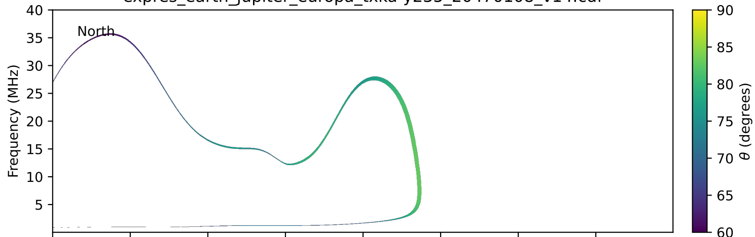
expres_earth_jupiter_europa_txka-y235_20470108_v14.cdf
