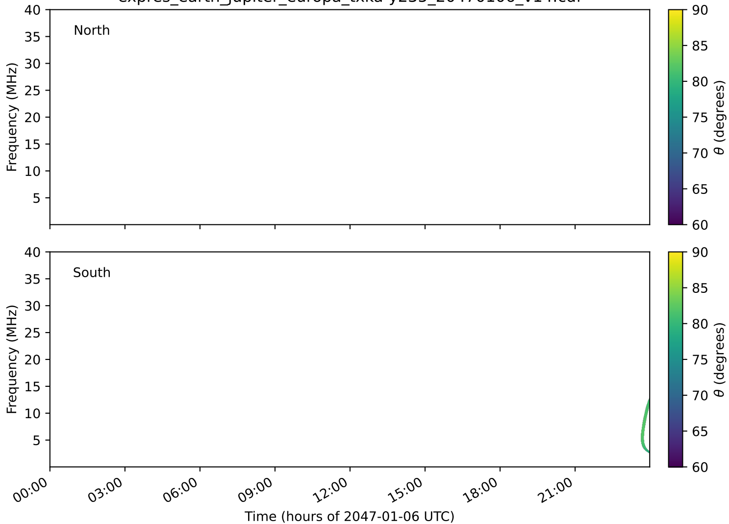
expres_earth_jupiter_europa_txka-y235_20470106_v14.cdf
