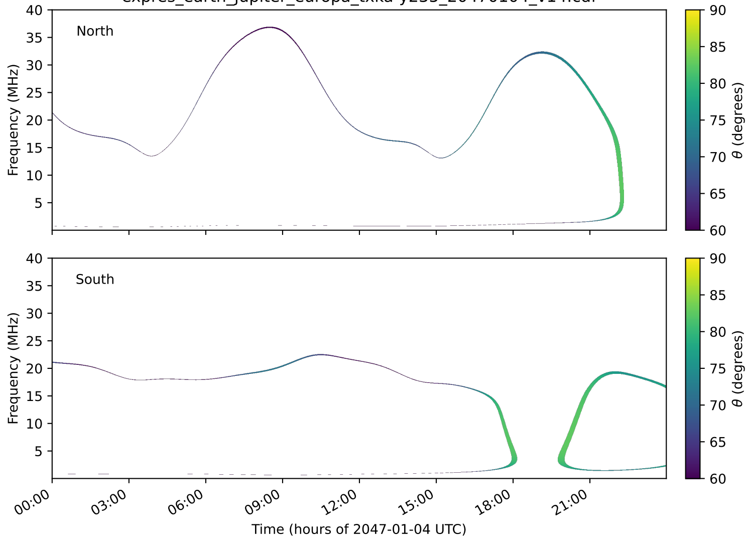
expres_earth_jupiter_europa_txka-y235_20470104_v14.cdf
