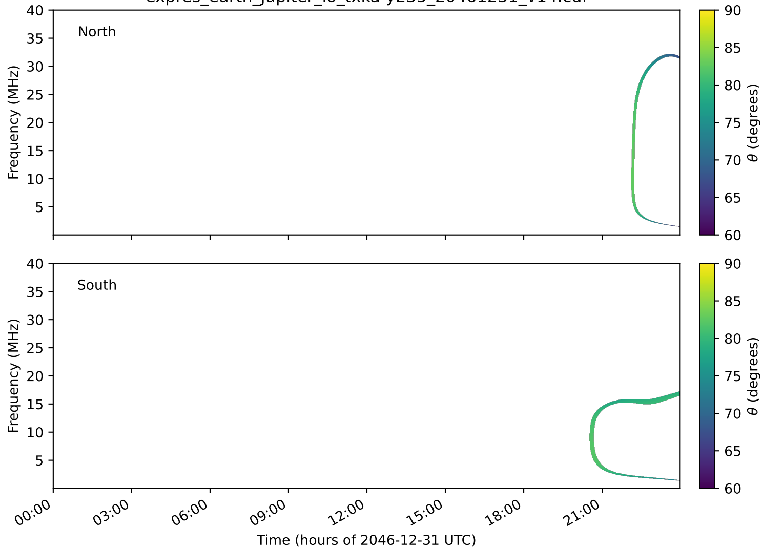
expres_earth_jupiter_io_txka-y235_20461231_v14.cdf
