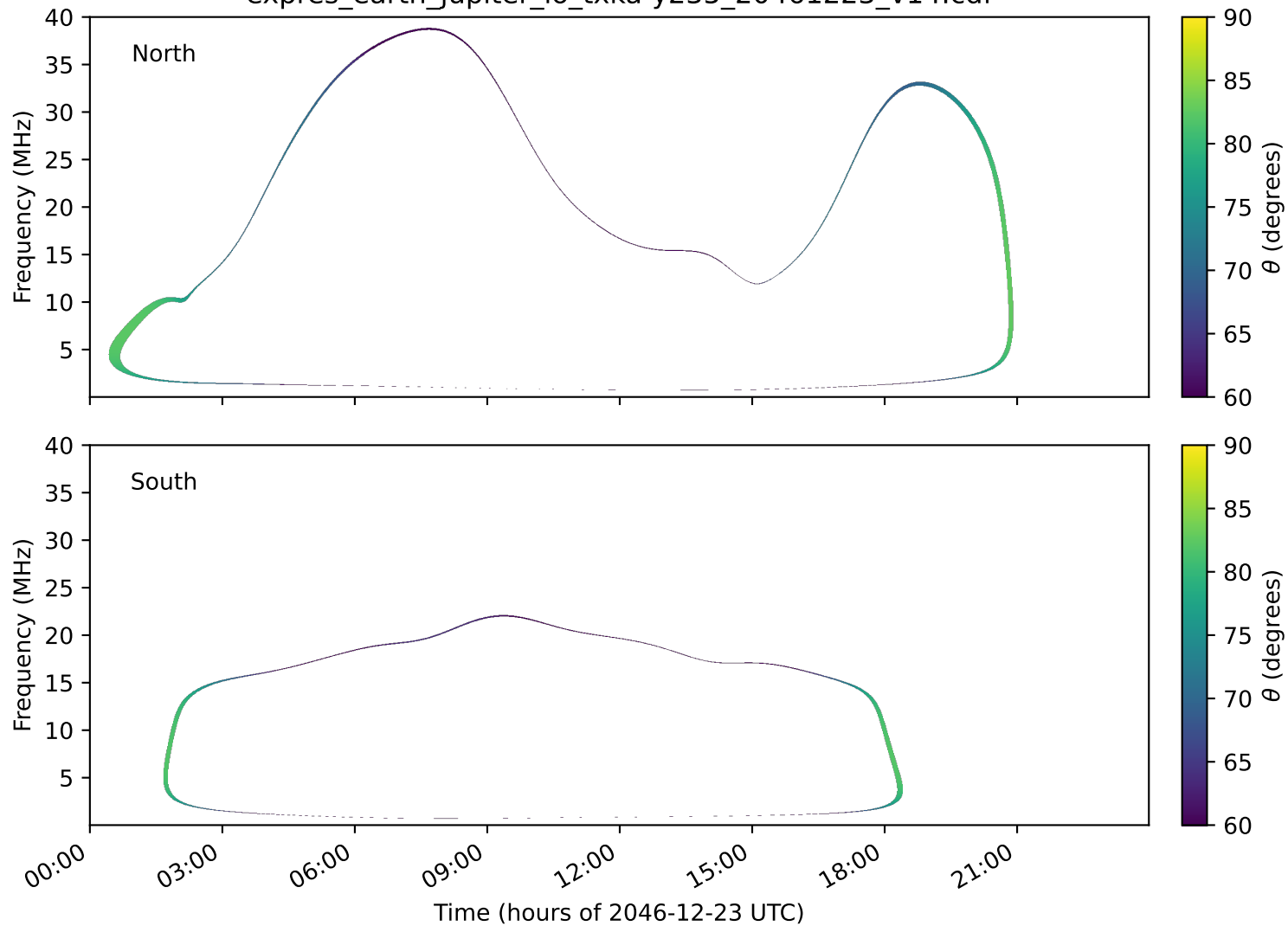
expres_earth_jupiter_io_txka-y235_20461223_v14.cdf
