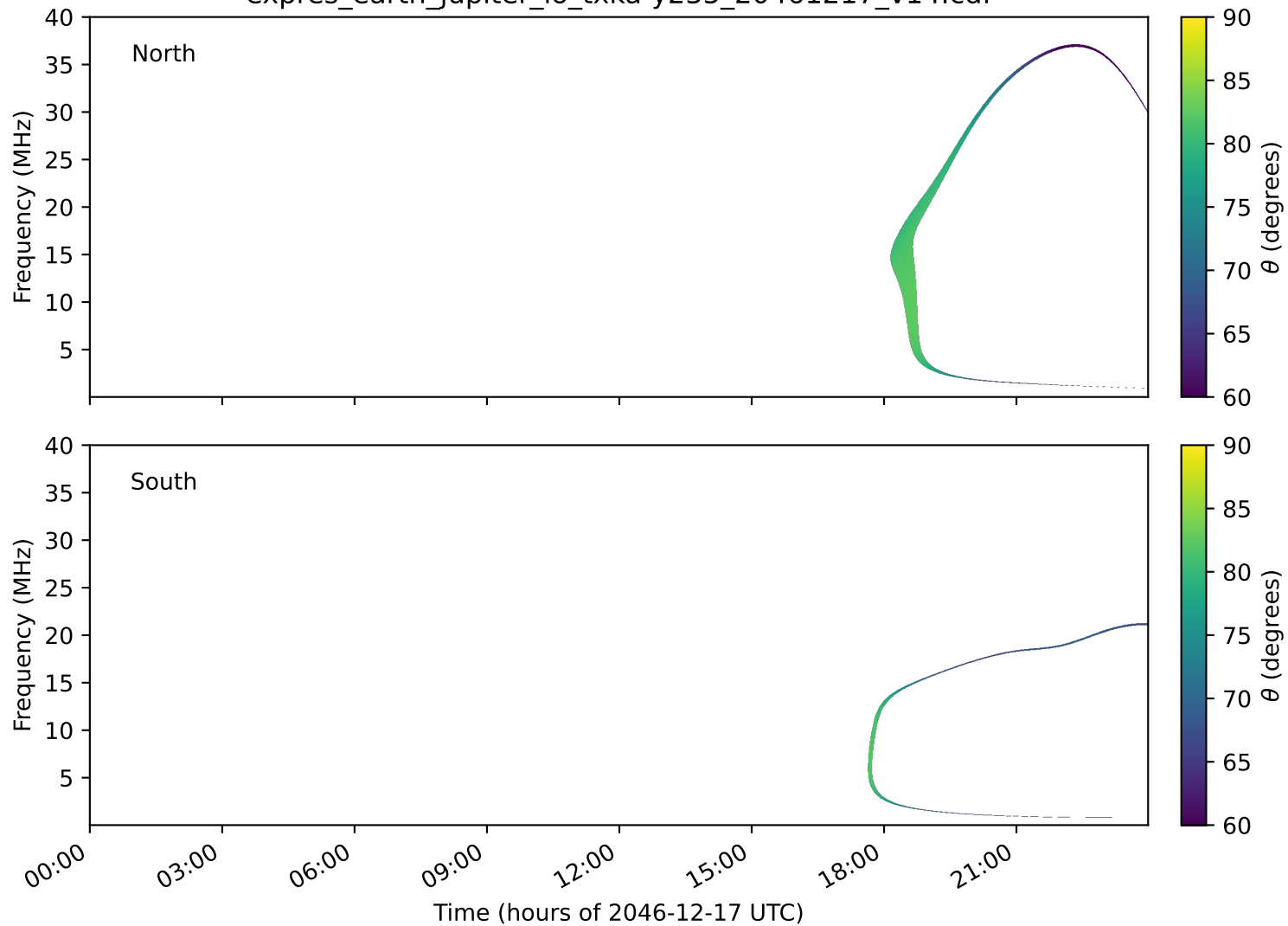
expres_earth_jupiter_io_txka-y235_20461217_v14.cdf
