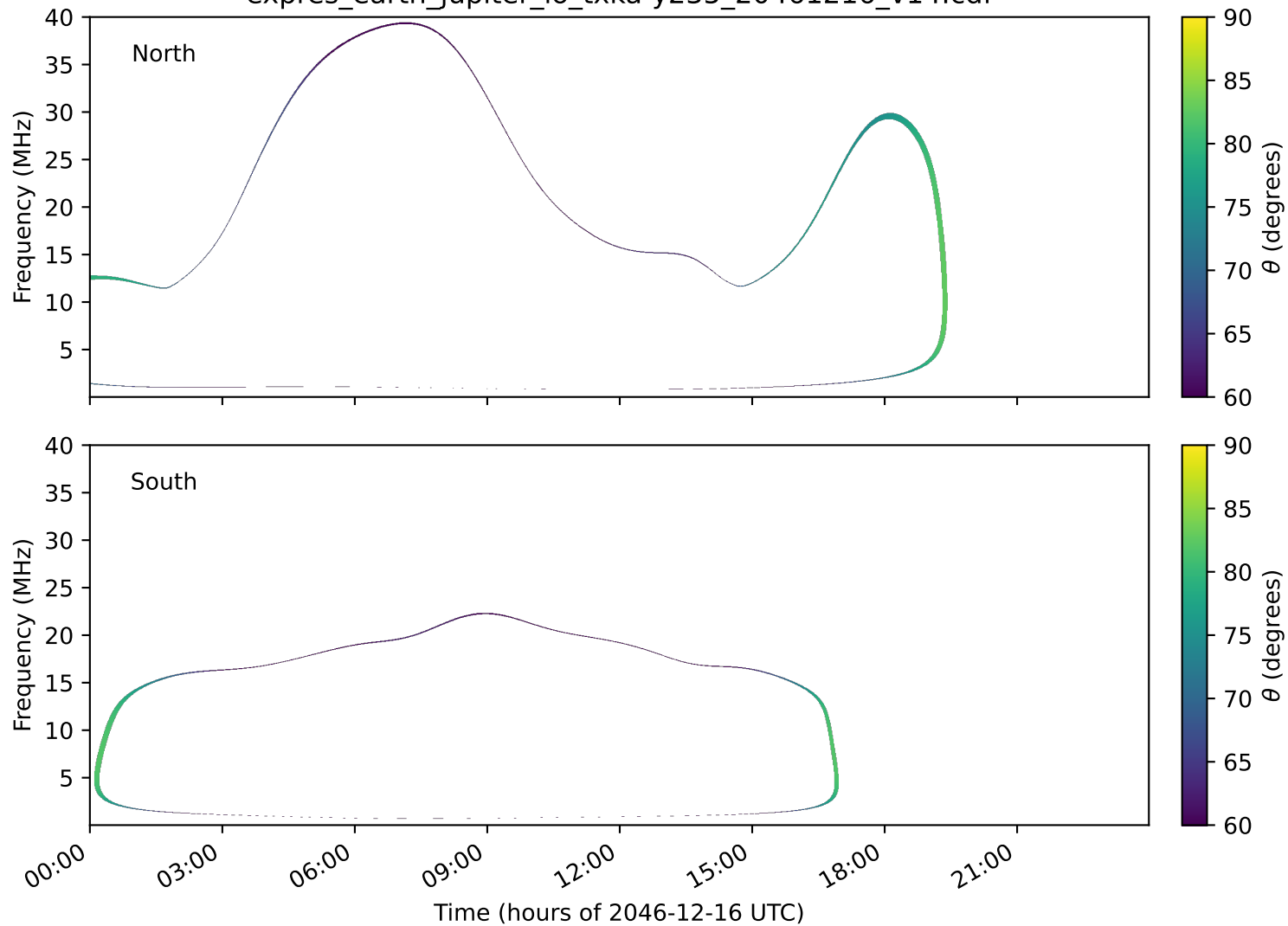
expres_earth_jupiter_io_txka-y235_20461216_v14.cdf
