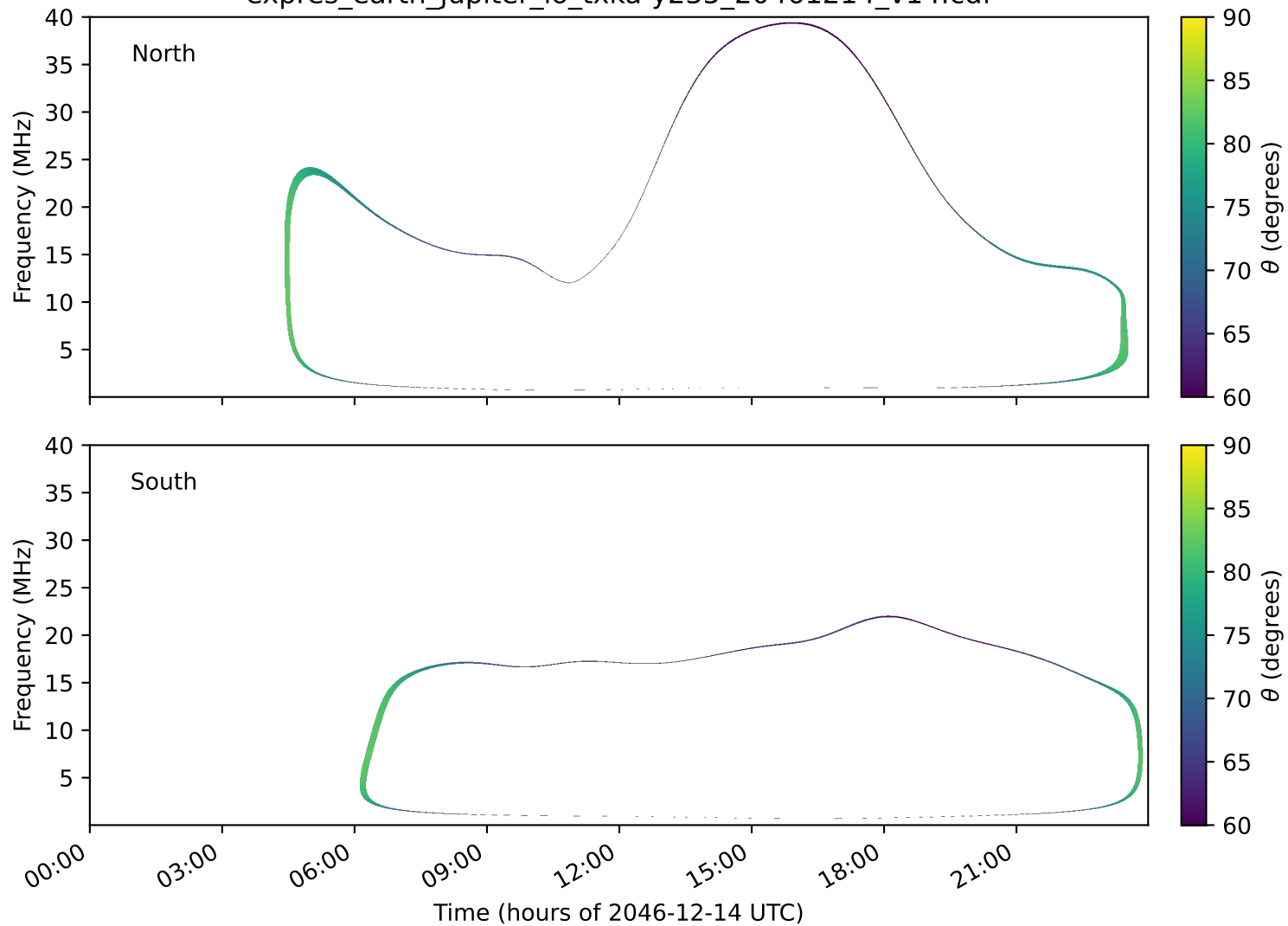
expres_earth_jupiter_io_txka-y235_20461214_v14.cdf
