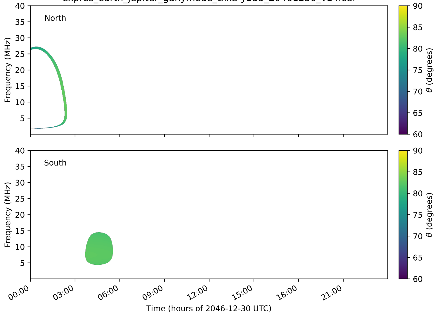
expres_earth_jupiter_ganymede_txka-y235_20461230_v14.cdf
