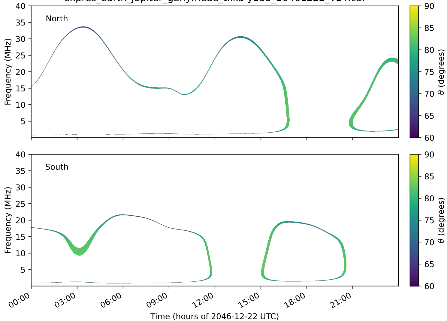
expres_earth_jupiter_ganymede_txka-y235_20461222_v14.cdf
