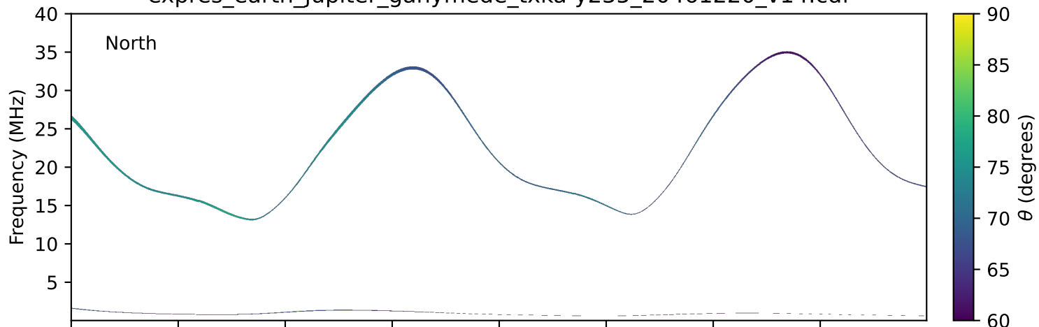
expres_earth_jupiter_ganymede_txka-y235_20461220_v14.cdf
