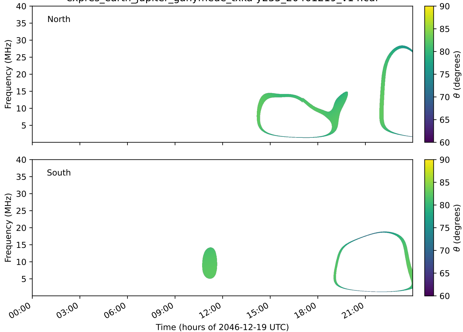
expres_earth_jupiter_ganymede_txka-y235_20461219_v14.cdf
