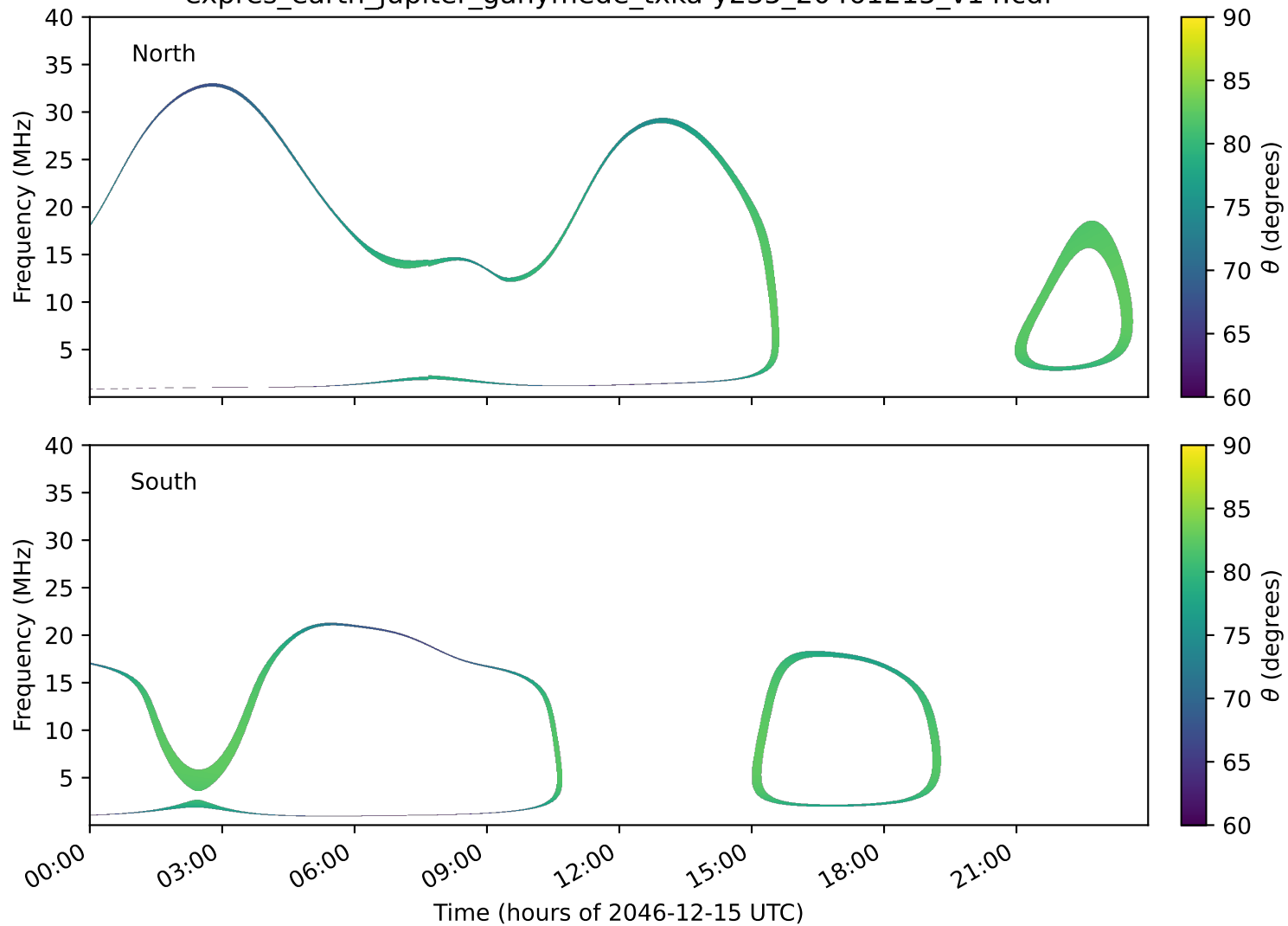
expres_earth_jupiter_ganymede_txka-y235_20461215_v14.cdf
