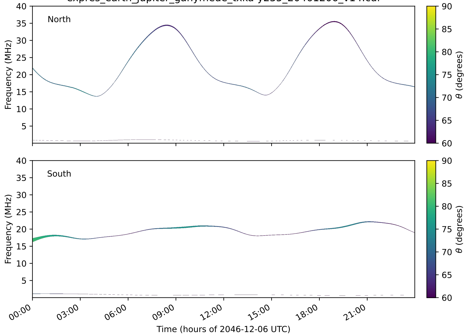
expres_earth_jupiter_ganymede_txka-y235_20461206_v14.cdf
