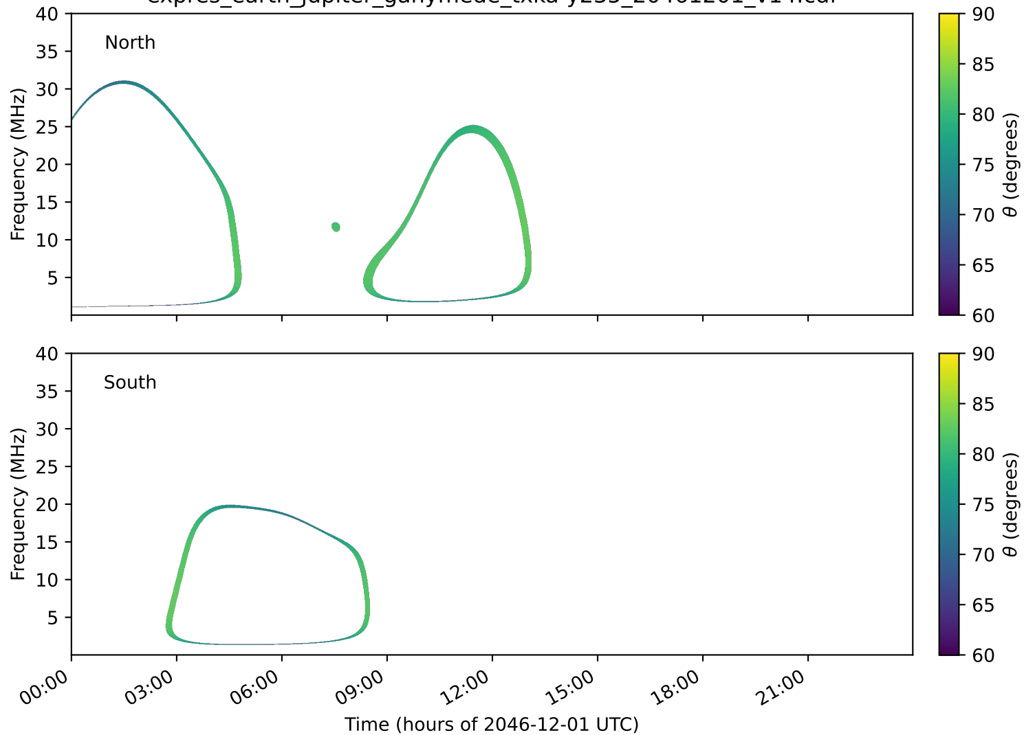
expres_earth_jupiter_ganymede_txka-y235_20461201_v14.cdf
