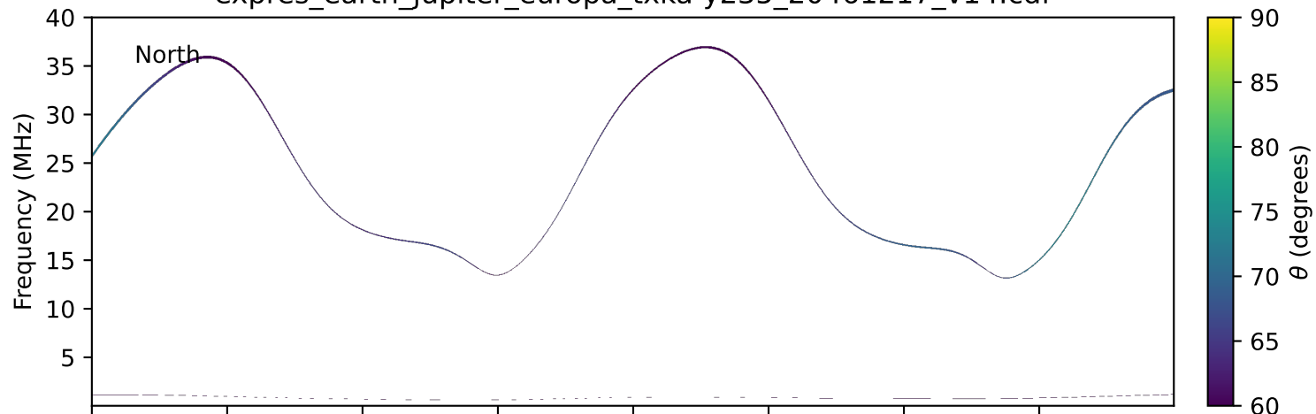
expres_earth_jupiter_europa_txka-y235_20461217_v14.cdf
