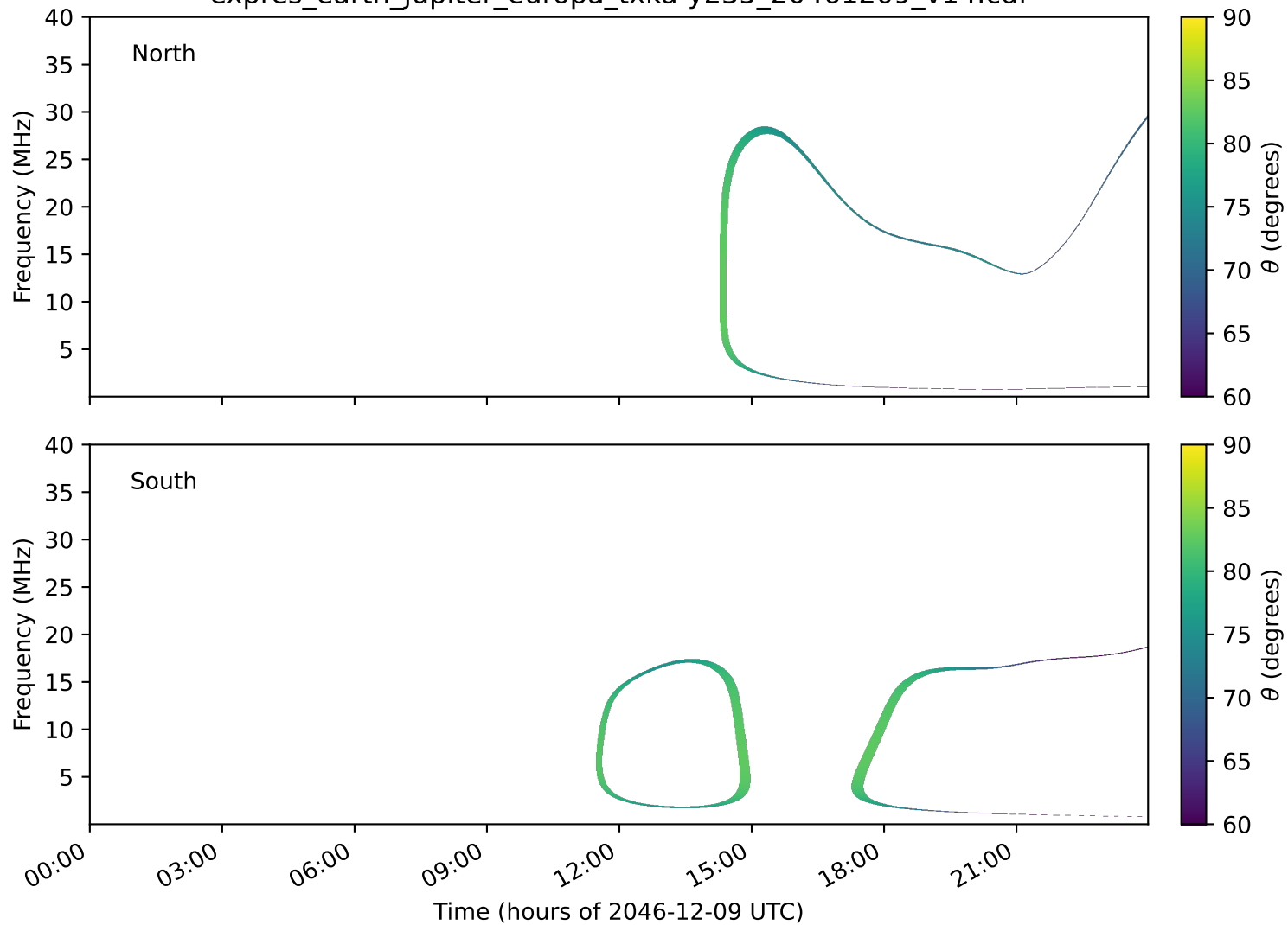
expres_earth_jupiter_europa_txka-y235_20461209_v14.cdf
