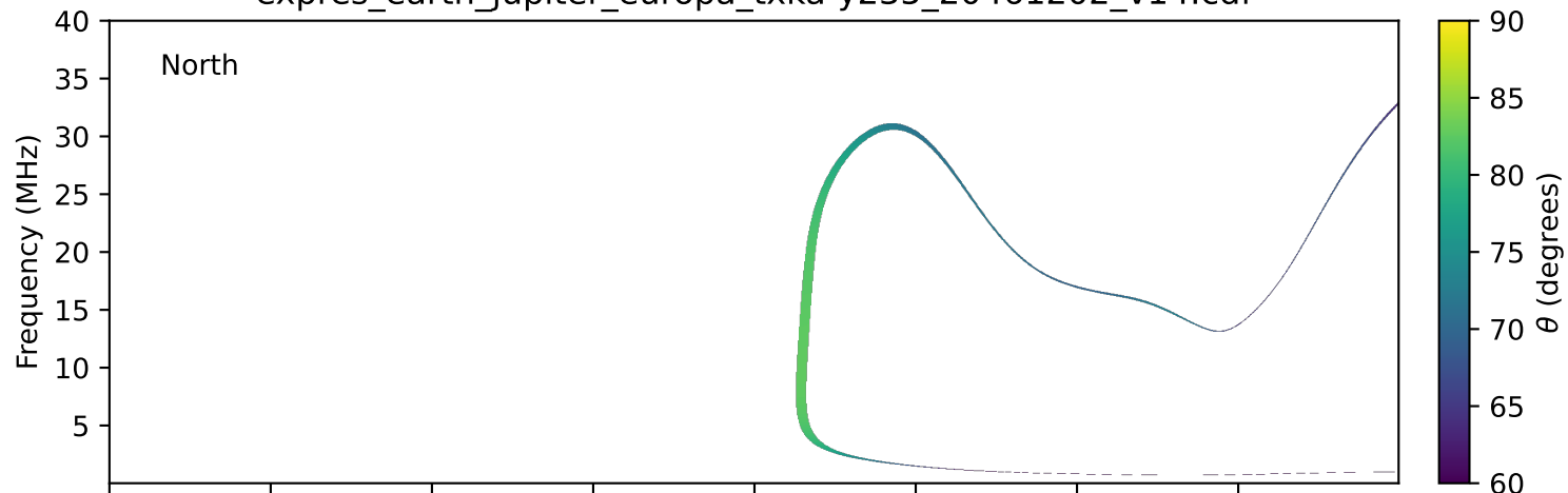
expres_earth_jupiter_europa_txka-y235_20461202_v14.cdf
