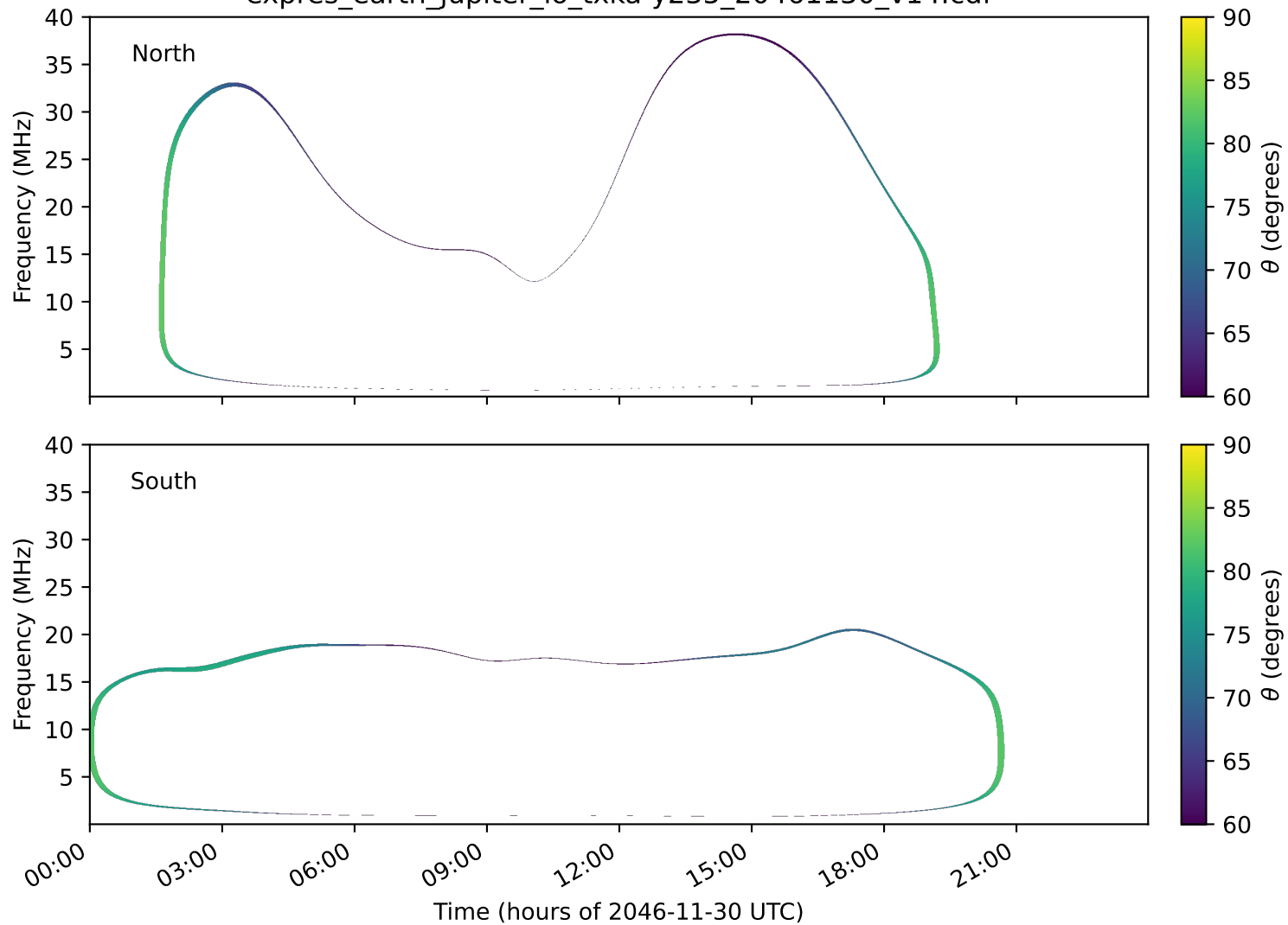
expres_earth_jupiter_io_txka-y235_20461130_v14.cdf
